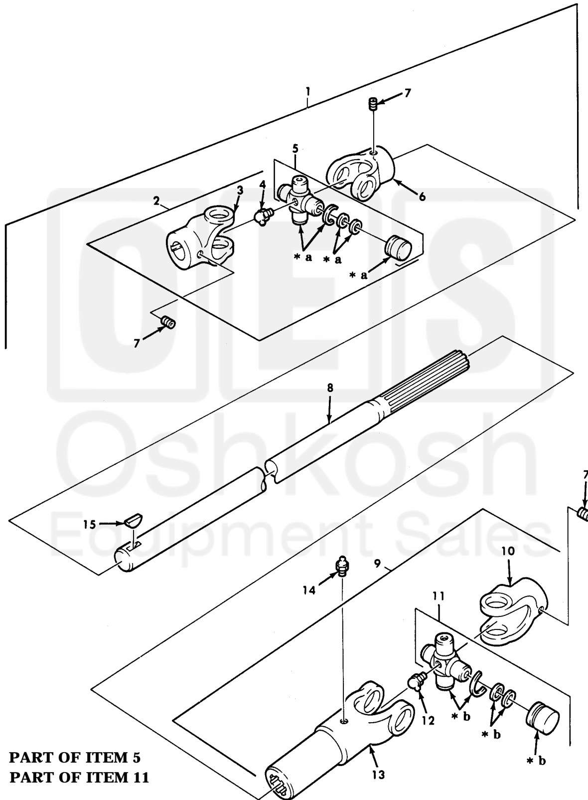
Figure 384. Dump Hoist Propeller Drive Shaft Assembly.
